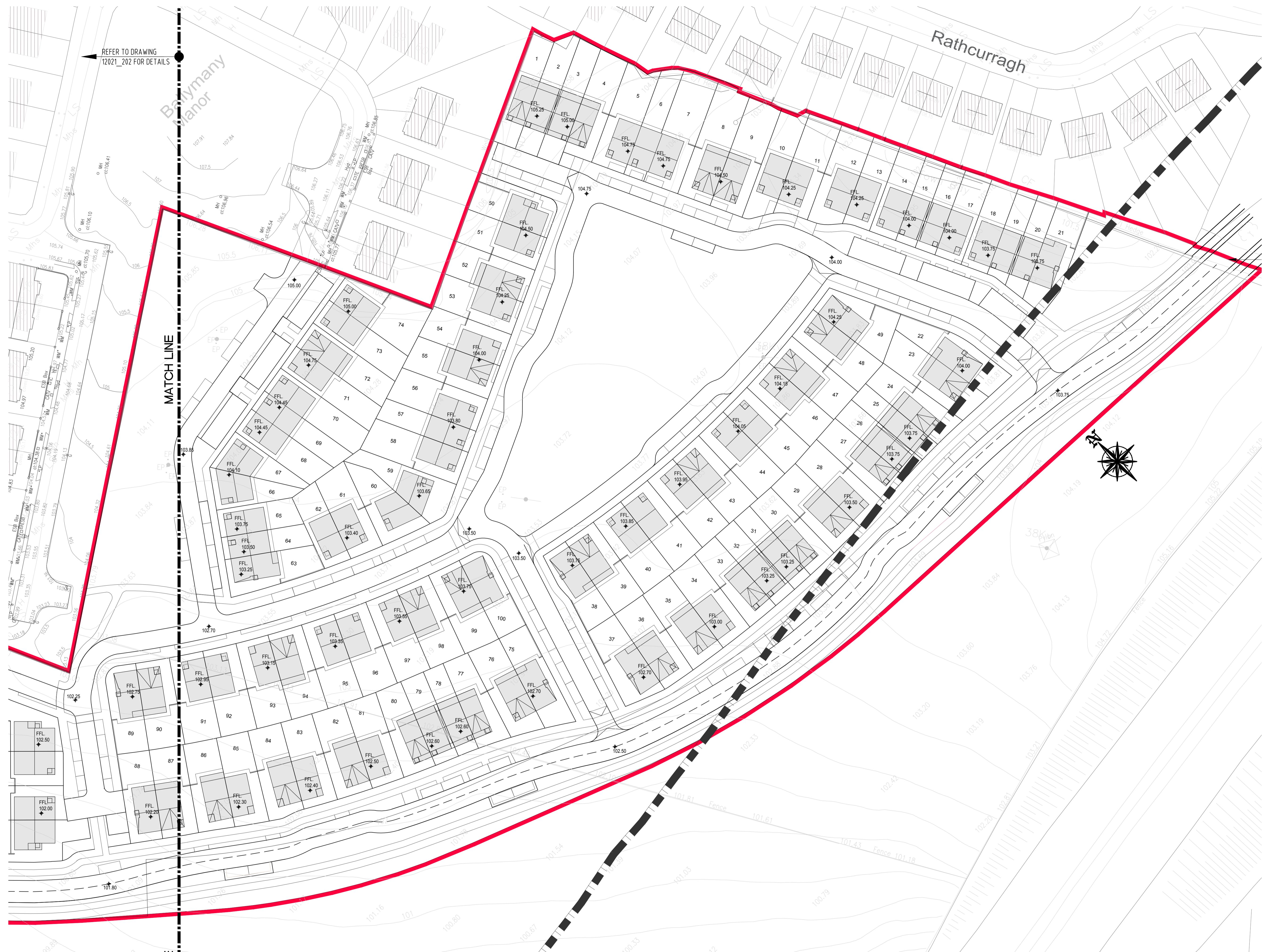
SITE LAYOUT SHOWING PROPOSED LEVELS (SHEET 2 OF 2) SCALE 1:500 AT A1
