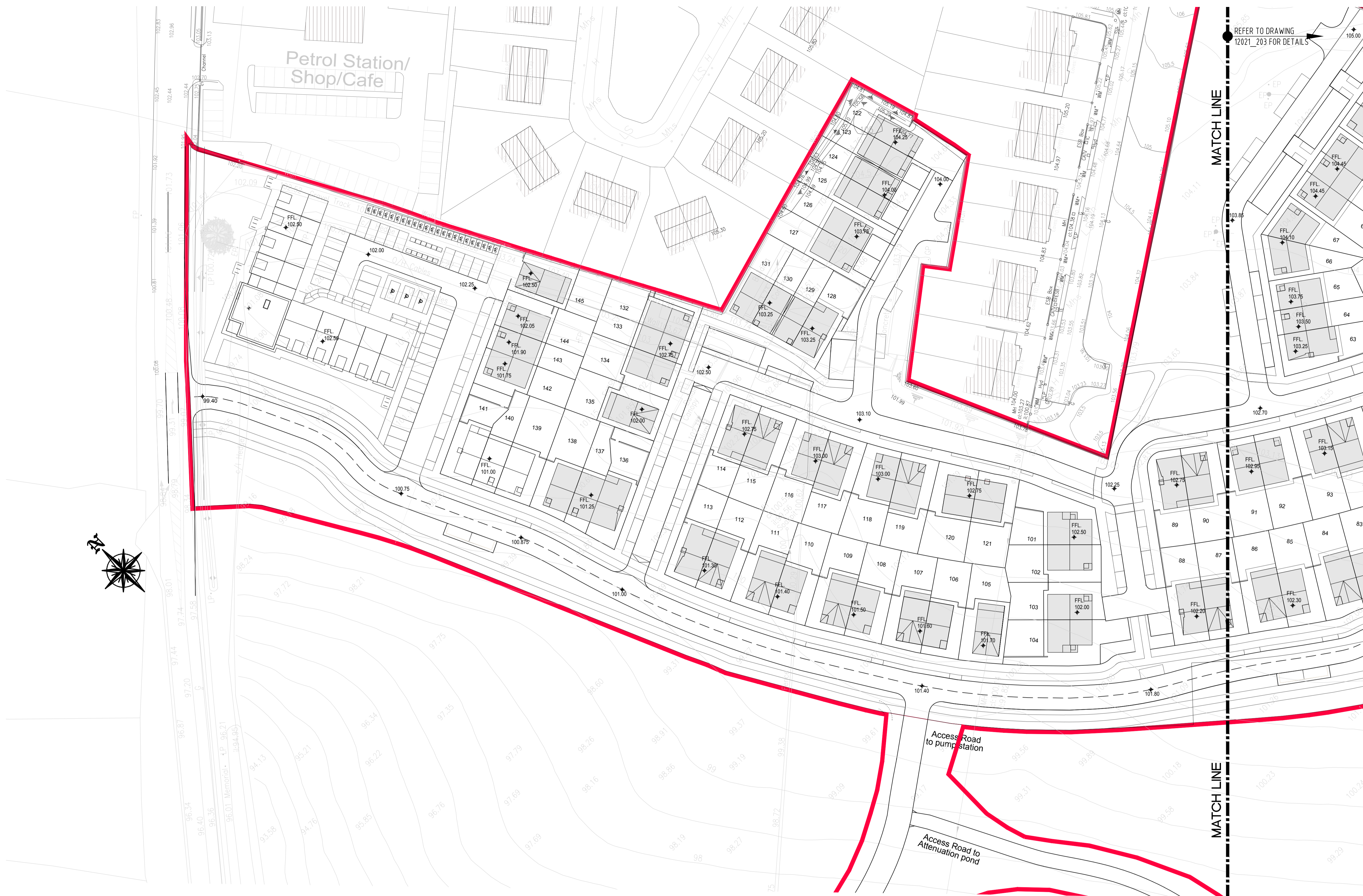
SITE LAYOUT SHOWING PROPOSED LEVELS (SHEET 1 OF 2) SCALE 1:500 AT A1
